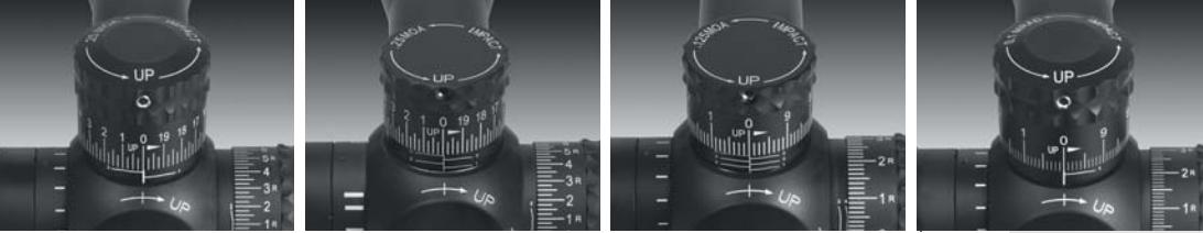
8-32 x 56 Hi-Speed Adjustments, L to R: .250 MOA with ZeroStop .250 MOA .125 MOA .1 Mil-Radian with ZeroStop
